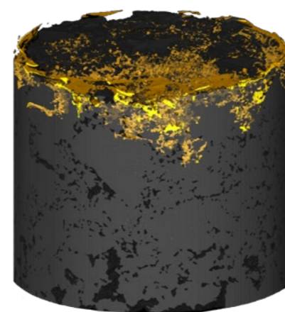
FIGURE 1 X-Ray CT scan on an Marshall Asphalt core showing the penetration of RHiNOPHALT® creating a reduction in porosity. The depth of penetration on this core sample is >15 mm.
